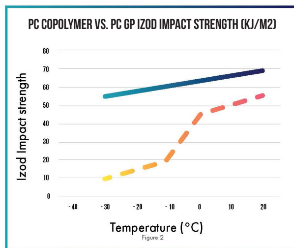
In Figure 1 and Figure 2, as temperature drops, general-purpose PC sees a noticeable decline in impact strength. Meanwhile, PC-SI maintains its strength, even as the temperature drops to extreme levels.
